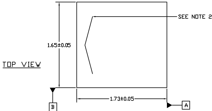
PACKAGE OUTLINE
