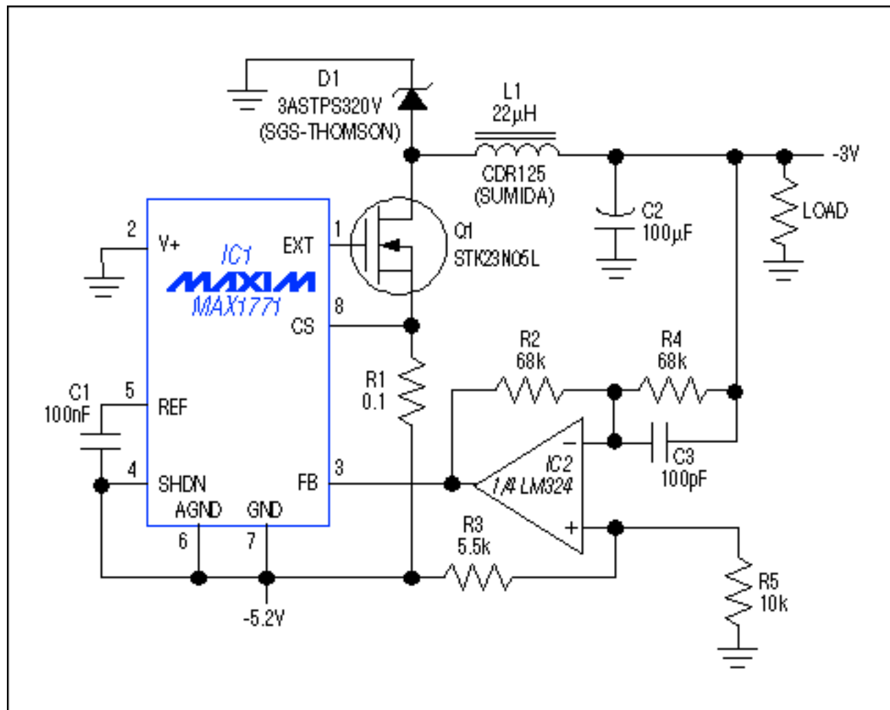
Figure 1. With an external op amp to invert its voltage feedback, this boost-mode dc-dc controller derives a regulated -3V from the -5.2V ECL supply.
