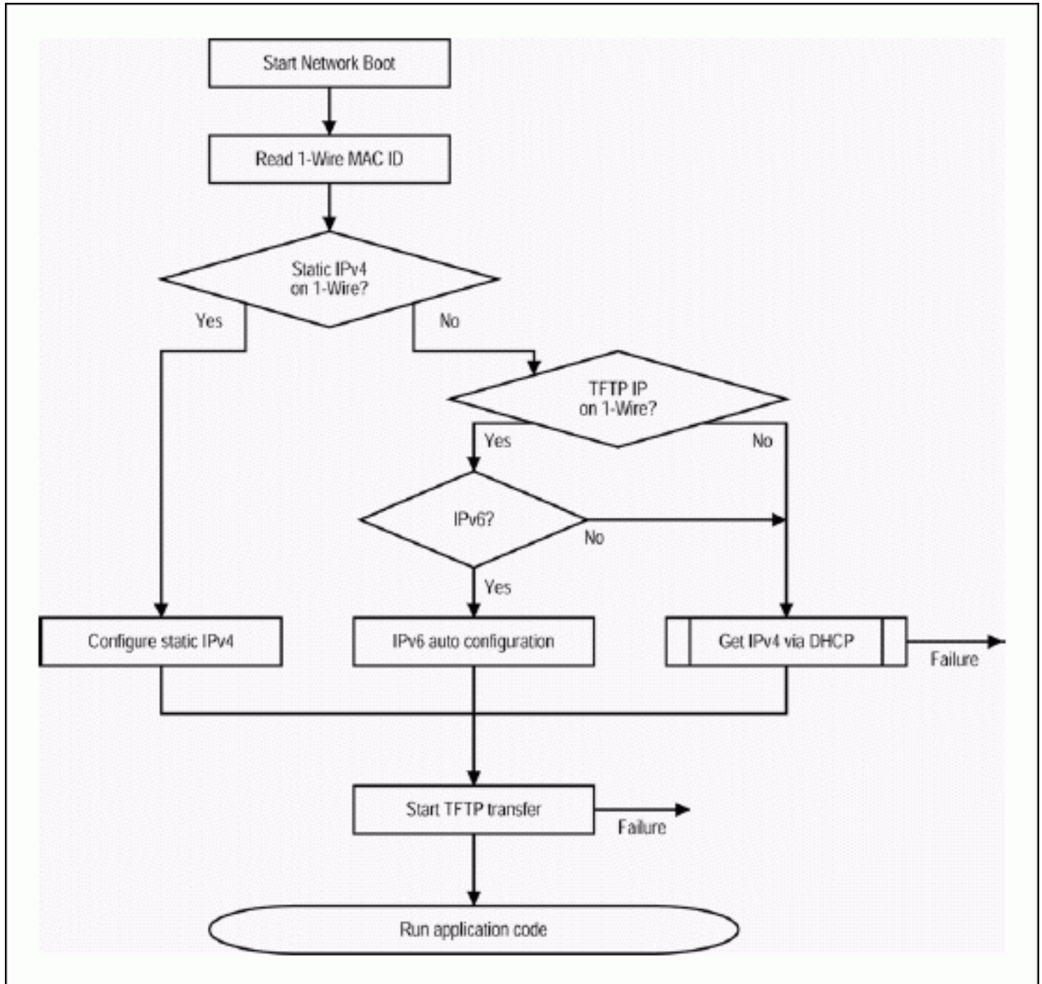
Figure 1. Network boot.
