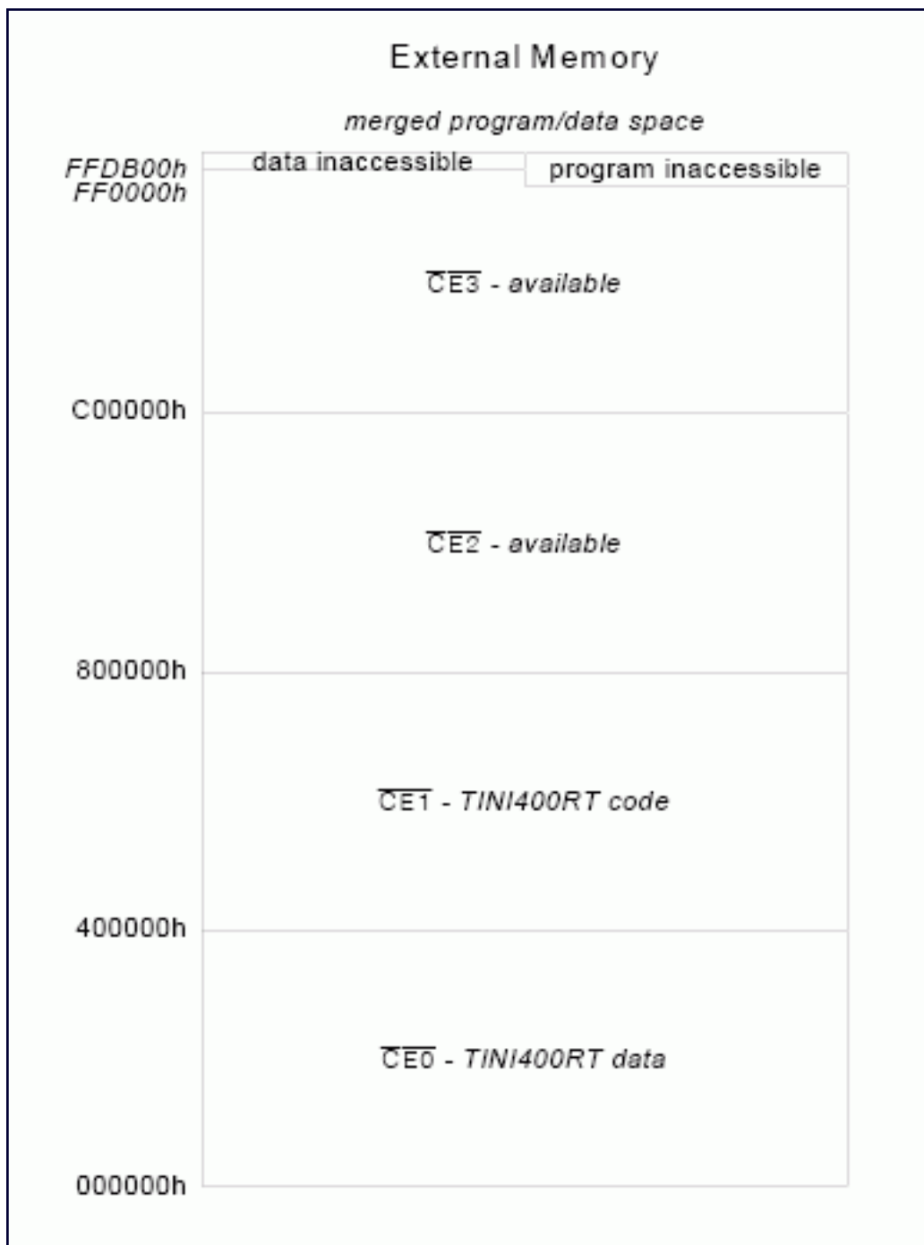
Figure 3. TINI400RT Memory Map with 4MB per Chip Enable.
