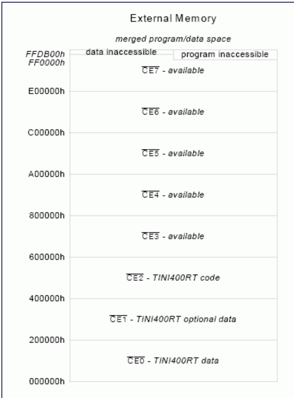
Figure 1. TINI400RT Memory Map
