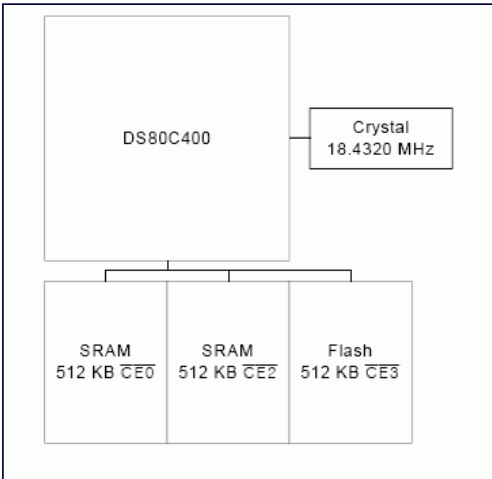
Figure 2. Example High-Speed Configuration.
