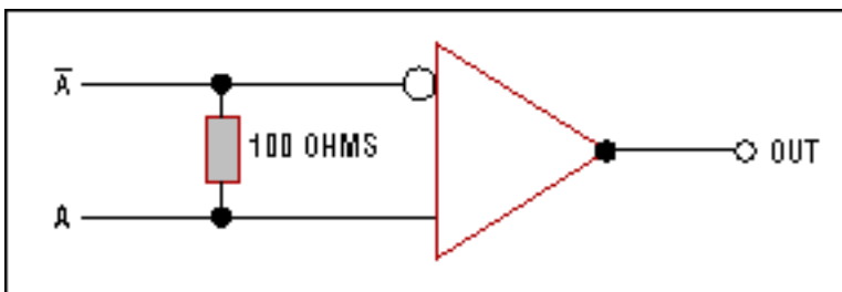
Figure 6. Receiver input connection.
