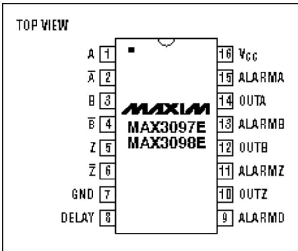
Figure 4. MAX3097 pinout.
