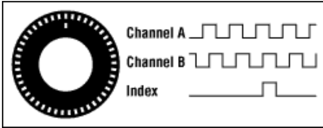
Figure 2. Optical encoder disk.
