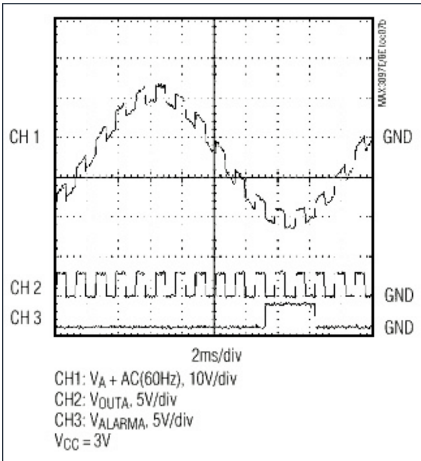
Figure 5. This shows the fault alarm on channel A due to the excessive common-mode range; the fault indicates that the data during this period can be unreliable.
