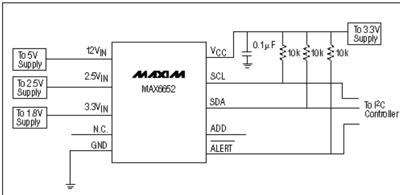
Figure 3. Circuit of Example 3. This circuit is used in a low-voltage system to monitor 5V, 3.3V, 2.5V, and 1.8V. The MAX6652 operates from a 3.3V supply. The 12V_{IN} input monitors the 5V supply, and the 3.3V_{IN} input monitors the 1.8V supply.
