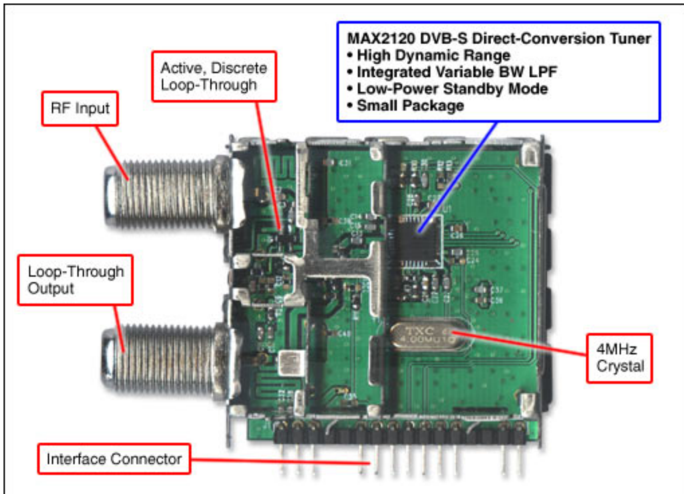
Figure 1. DVB-S Half-NIM reference design features the MAX2120 tuner.
