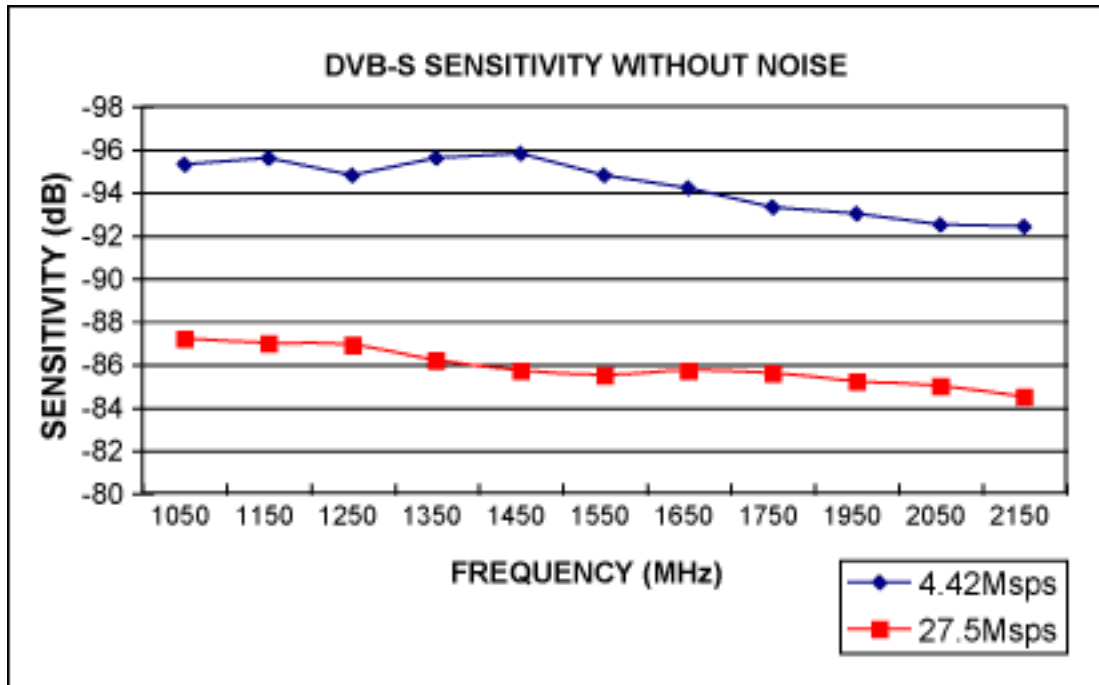
Figure 3. The DVB-S sensitivity without noise is better than -92.5dBm for 4.42Mps, and better than -84dBm for 27.5Mps across the band.
