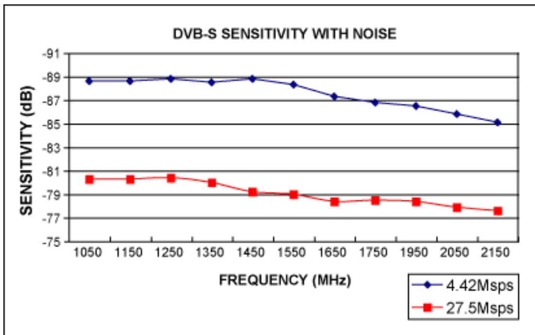
Figure 4. When noise is added, the DVB-S sensitivity is better than -85dBm for 4.42Mps, and better than -77.5dBm for 27.5Mps across the band. For this case, AWGN noise is added with C/N = 5dB. For the 4.42Mps data rate, the noise bandwidth is 5.7MHz; for the 27.5Mps data rate, the noise bandwidth is 35.2MHz.
