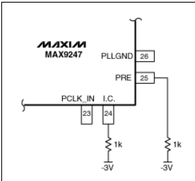
Figure 1. Two resistors bias the MAX9247 into test mode.
