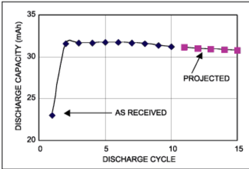
Figure 6. ML2020R capacity vs. discharge cycle.
