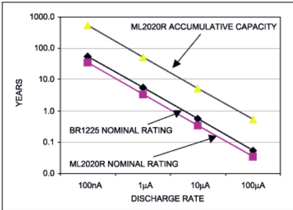
Figure 7. Accumulative lifetime capacity.
