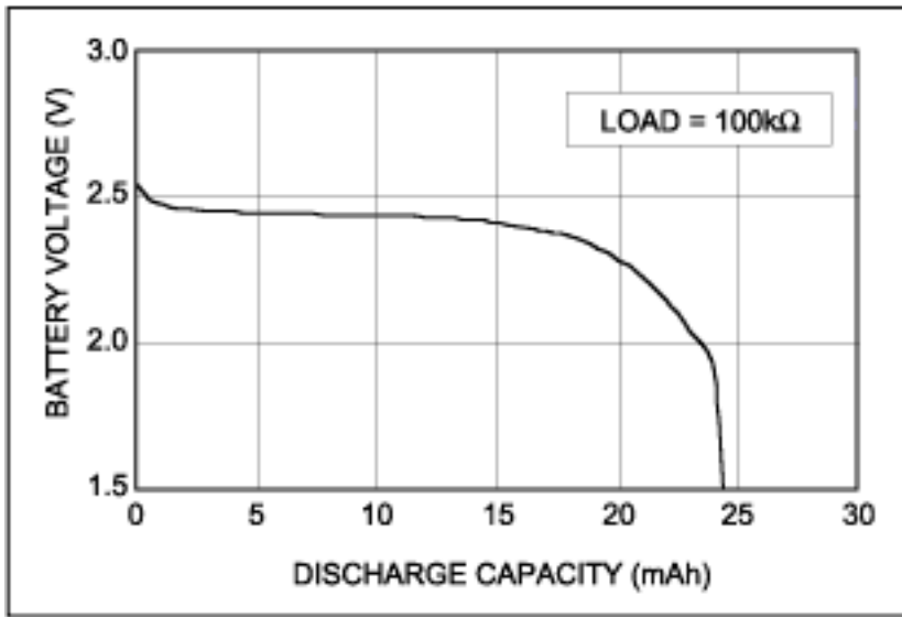
Figure 3. ML2020R "As Received" capacity.
