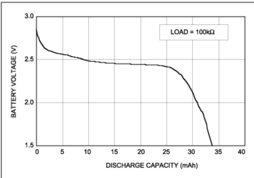
Figure 5. ML2020R capacity after a full charge.
