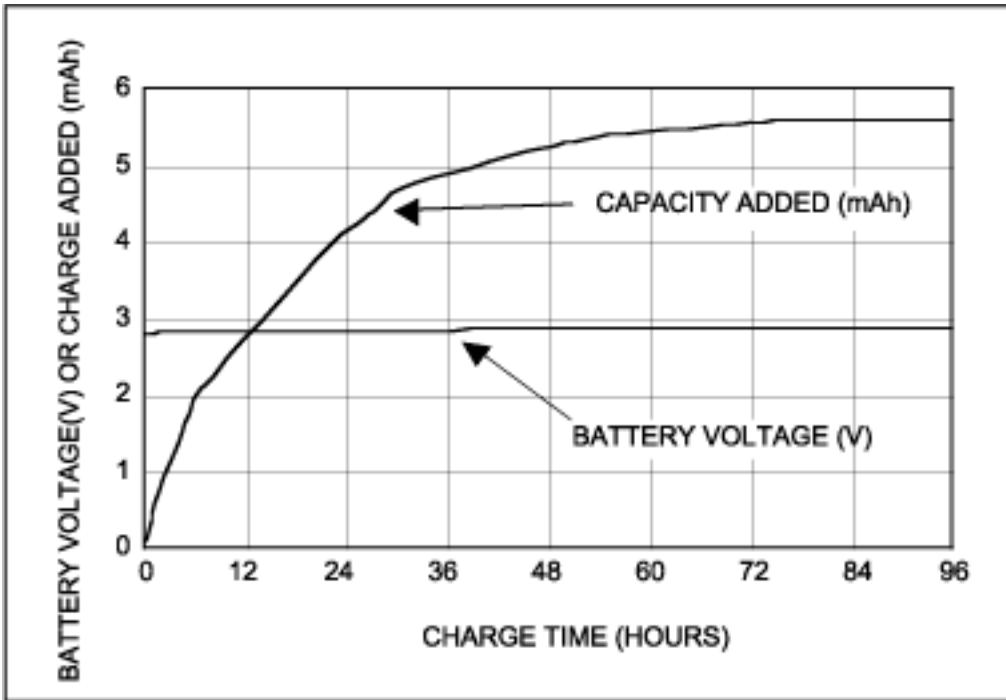
Figure 4. Initial charge profile for a ML2020R battery.
