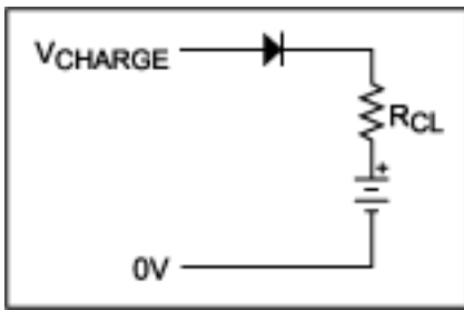
Figure 2. Charge circuit for an ML battery.
