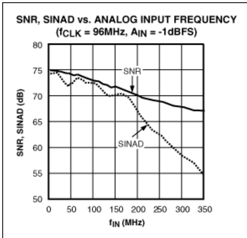
Figure 1. The SNR and SINAD for the 96Msps MAX1259 ADC are plotted vs. input frequency at a clock rate of 96MHz and an amplitude level of -1dBFS.
