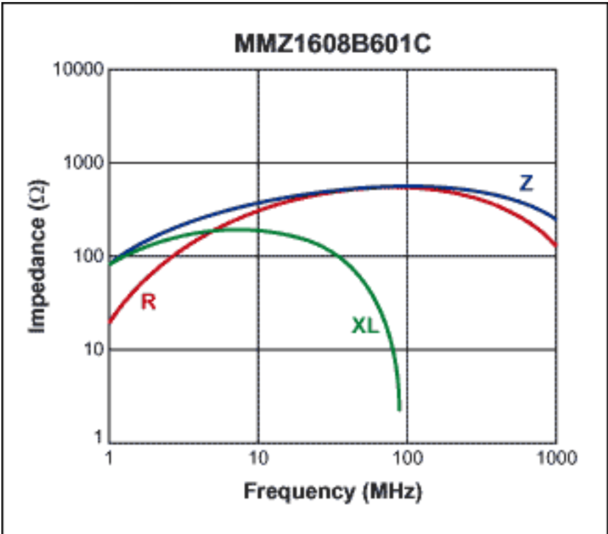
Figure 3. Impedance vs. frequency curve for the TDK MMZ1608B601C ferrite bead.
